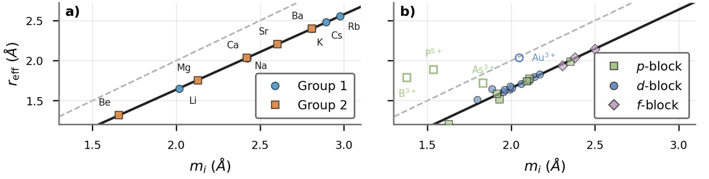
FIG. 2. First-principles screening centroid r_{\text{eff}} vs. Gibbs shell centroid m_i . (a) Ten s -block ground-state binary oxides. The solid line is the shared fit and the dashed line is r_{\text{eff}} = m_i . (b) Twenty-five non- s -block ground-state binary oxides, color-coded by block. Open symbols mark the four directional-bonding outliers excluded from the regression ( \text{B}_2\text{O}_3 , \text{P}_2\text{O}_5 , \text{As}_2\text{O}_3 , \text{Au}_2\text{O}_3 ).
