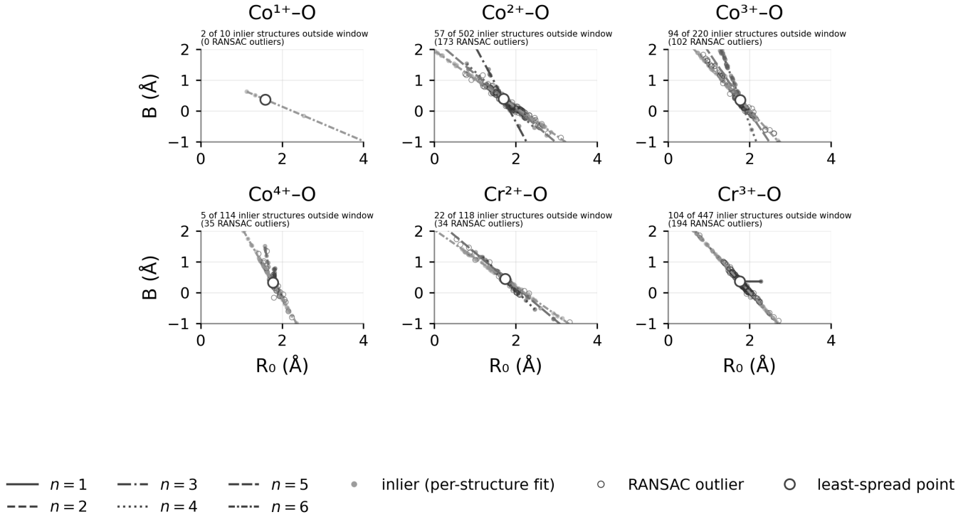
FIG. S4. n -resolved B vs. R_0 for oxidation-state-resolved 3d X-O pairs ( Co^{1+} , Co^{2+} , Co^{3+} , Co^{4+} , Cr^{2+} , Cr^{3+} ).
