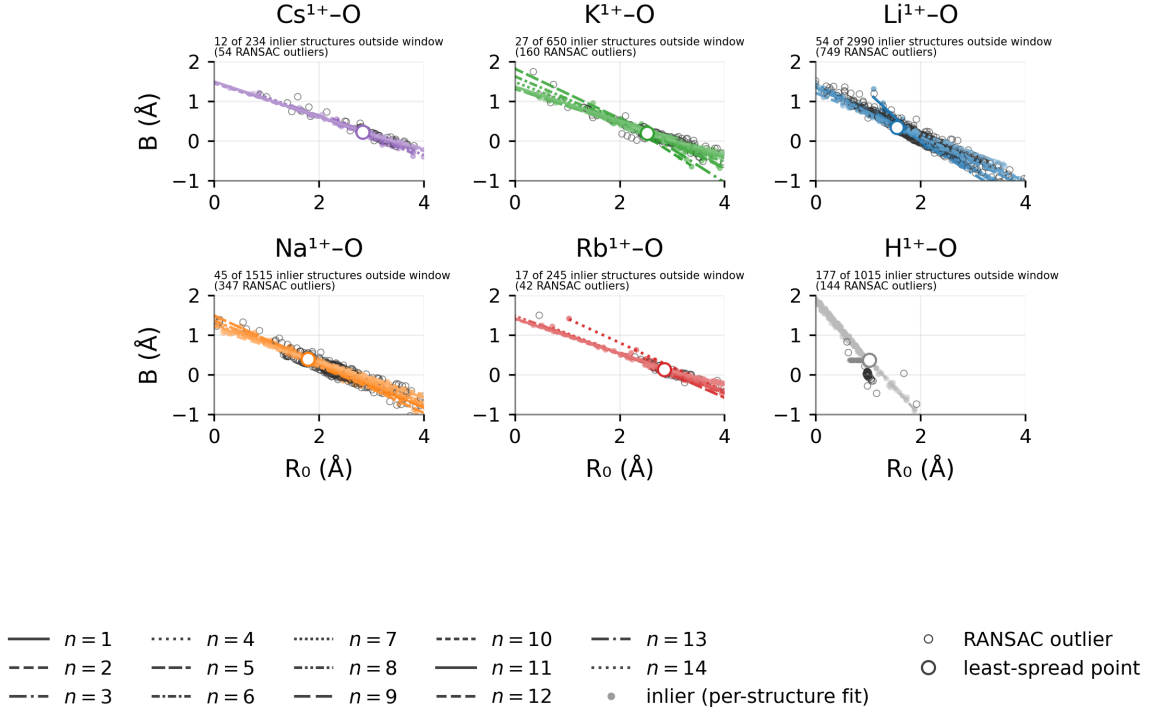
FIG. S2. n -resolved B vs. R_0 fit lines for Group 1 X-O pairs (Cs, K, Li, Na, Rb, H). Line-Filled circles are the per-structure (R_0, B) inliers of each line, open circles the RANSAC outliers, line styles distinguish coordination numbers n (legend), and the large open circle marks the least-spread intersection point. Axes are fixed to 0 < R_0 < 4 Å and -1 < B < 2 Å, with the number of inlier structures outside the window given above each panel. The convergence of the lines defines the characteristic pair (R_0^*, B^*) for each cation.
