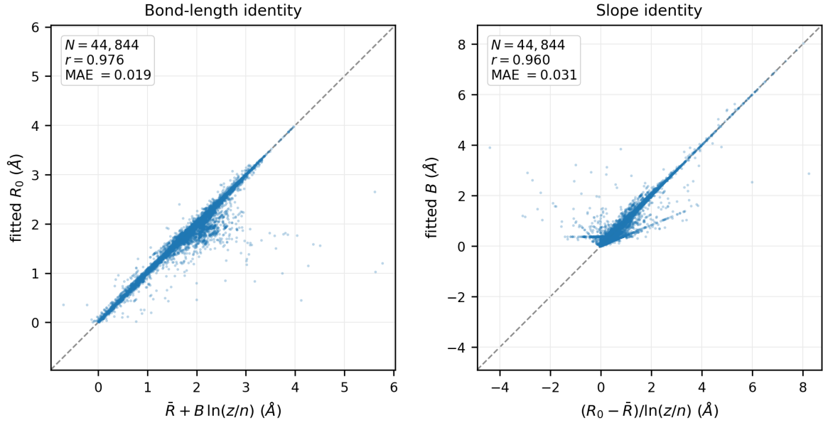
FIG. S19. Left: parity between fitted R_0 and \bar{R}_0 + B \ln(z/n) for 44,844 screening-branch cation–oxygen structures. Right: parity between fitted B and (R_0 - \bar{R}_0)/\ln(z/n) for the same set.
