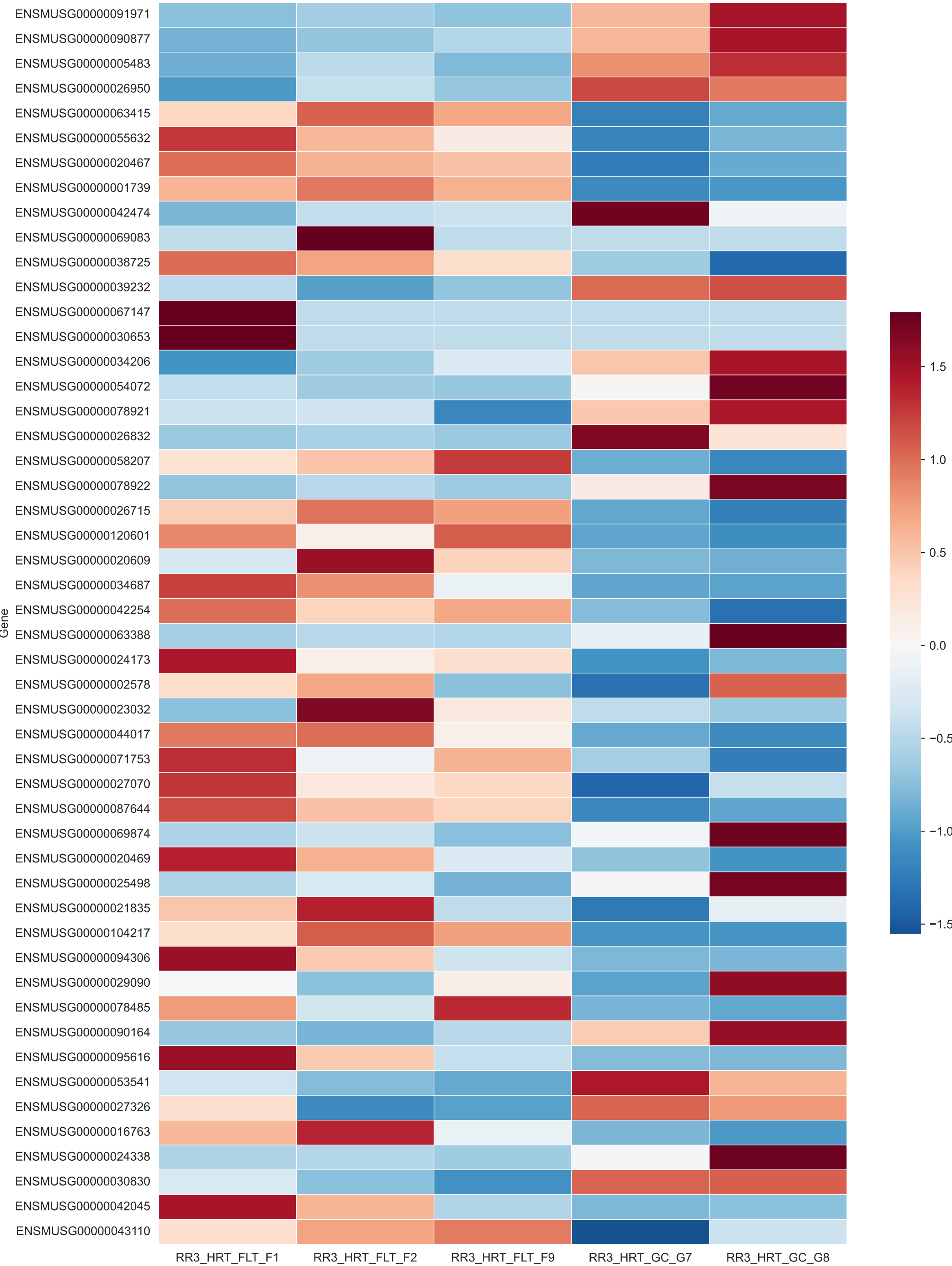
Top 50 DEGs - OSD-270
