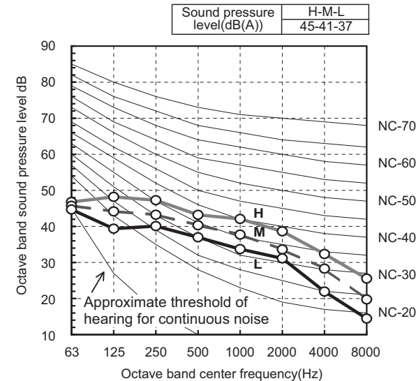
MMU-AP0244SH-E
