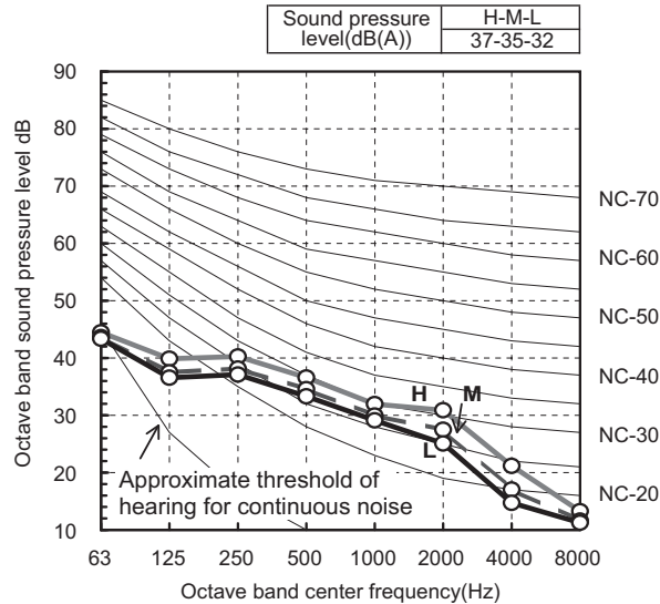
MMU-AP0244SH-E
