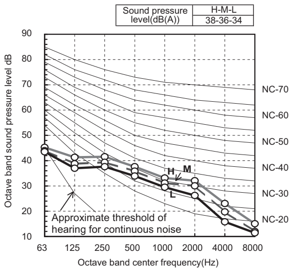
MMU-AP0184SH-E
