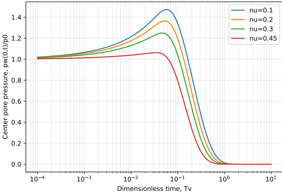
Cryer analytical center-pressure reference
