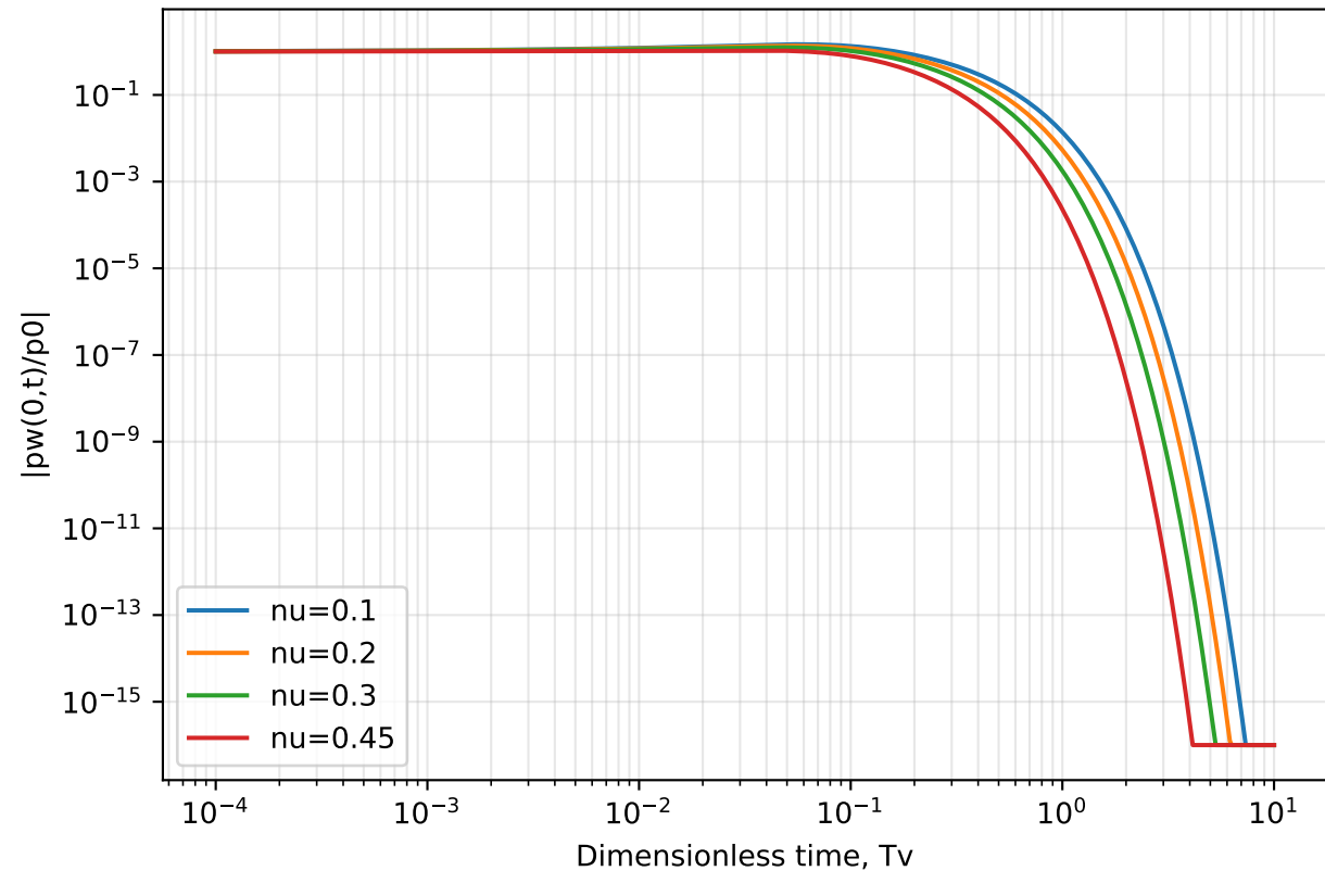
Cryer analytical long-time decay
