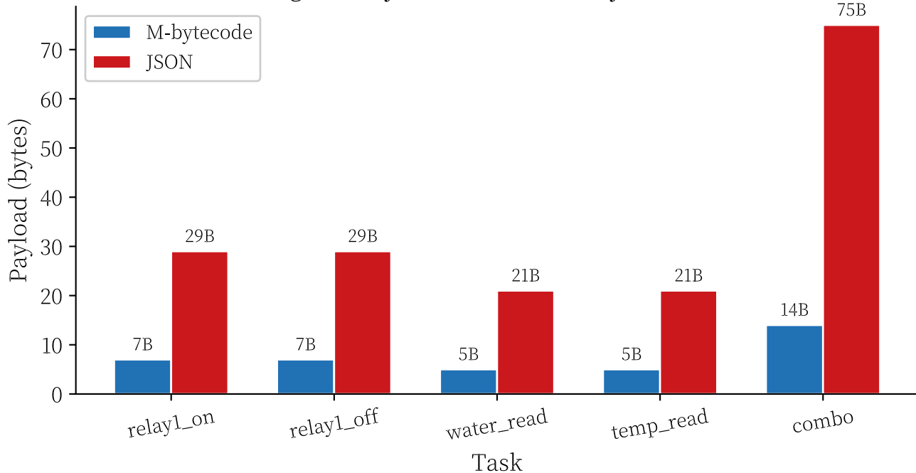
Fig.6 M-bytecode vs JSON Payload Size
