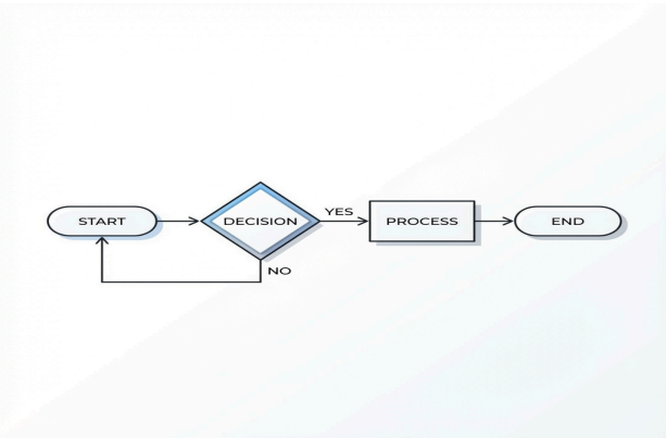
3. Flowchart (Expected: ?)
