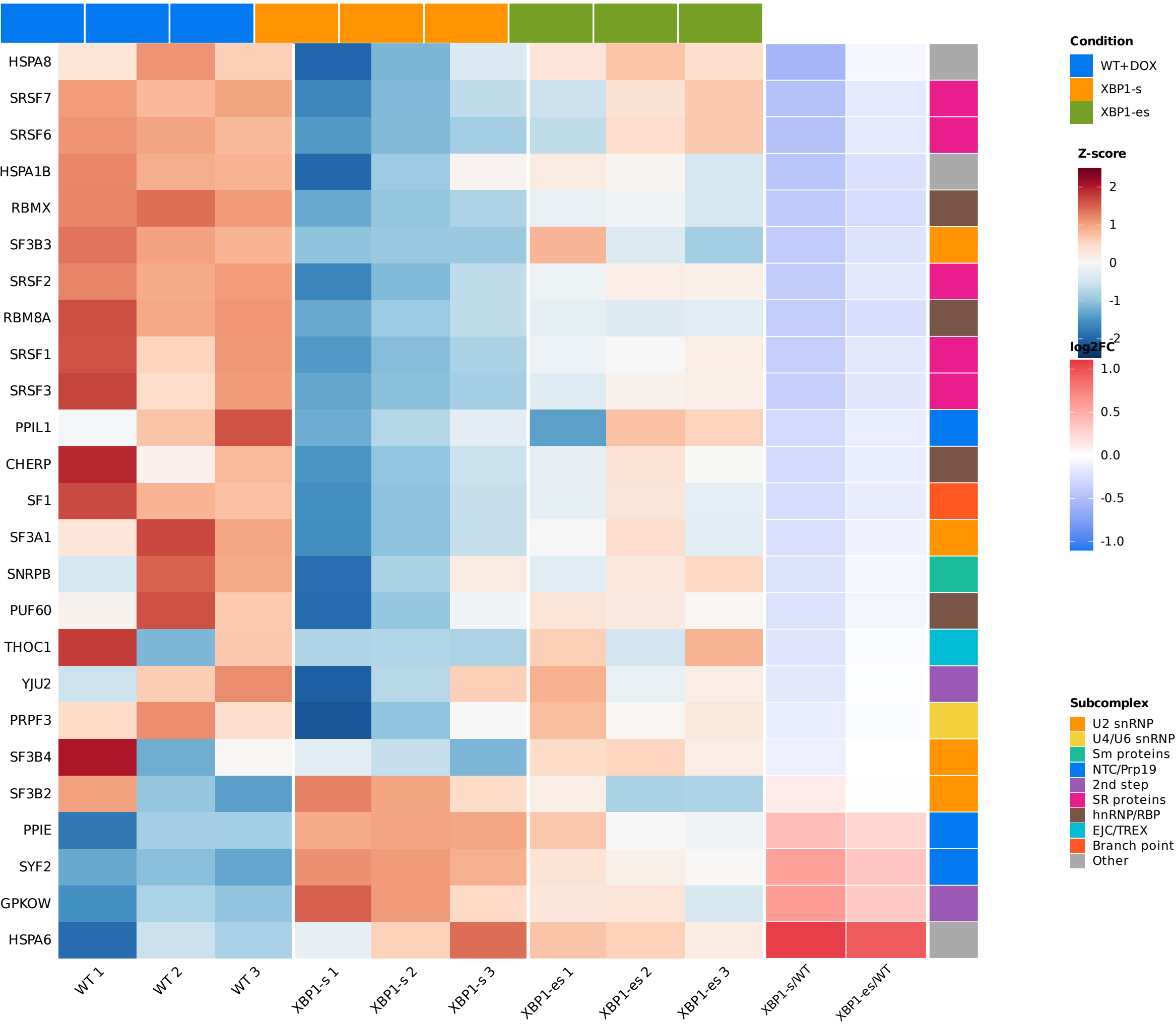
Spliceosome genes - biggest change in XBP1-s (not XBP1-es), top 25
