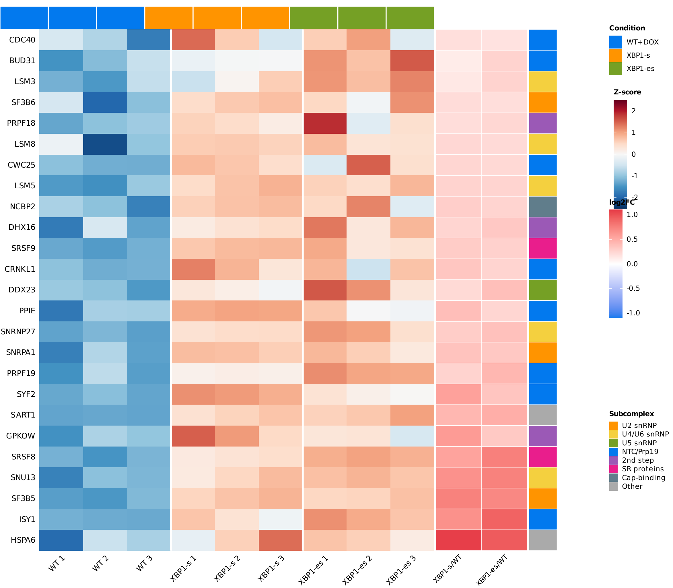
Spliceosome genes - upregulated in both XBP1-s and XBP1-es vs WT, top 25
