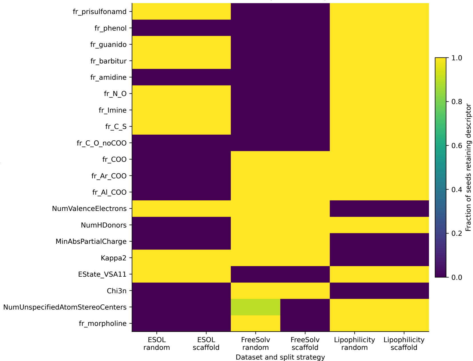
Most variable train-only RDKit descriptor retention
