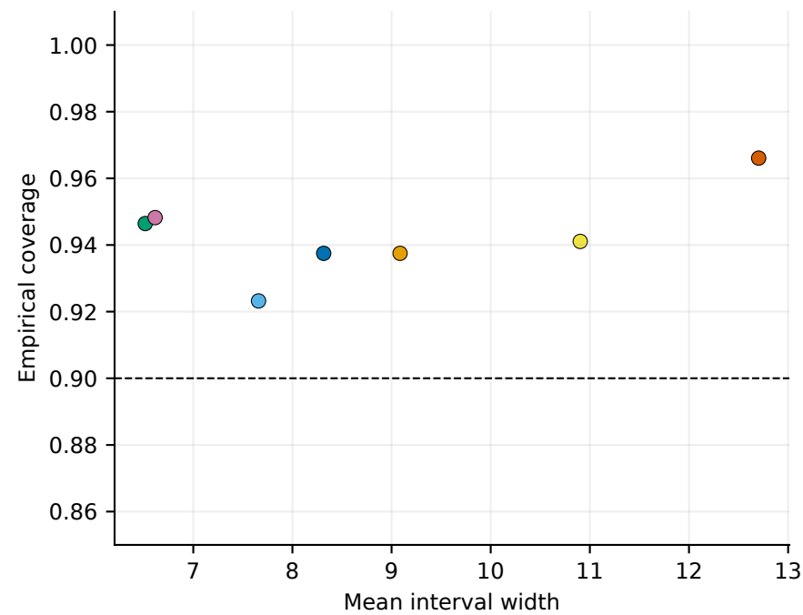
FreeSolv — scaffold
