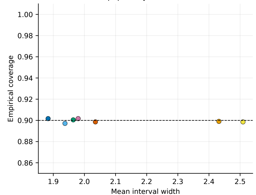
Lipophilicity — scaffold
