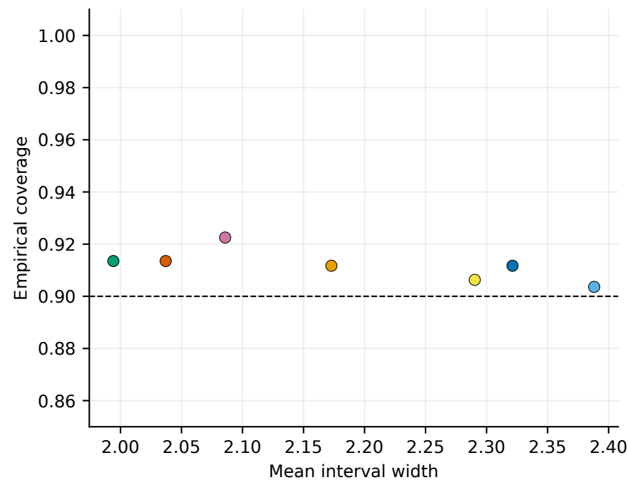
ESOL — scaffold
