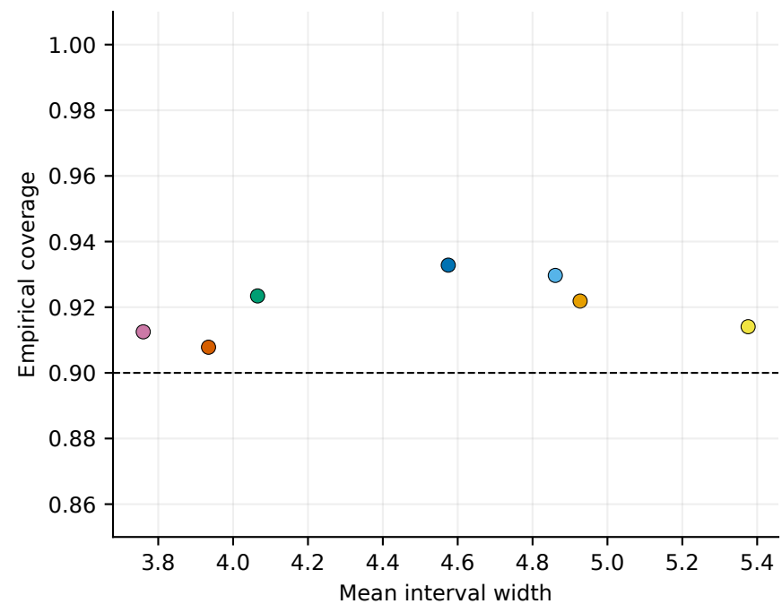
FreeSolv — scaffold
