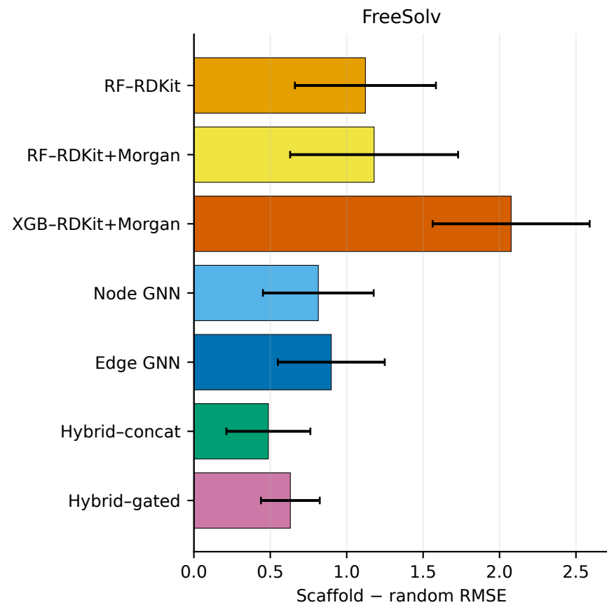
Generalization penalty under scaffold shift
