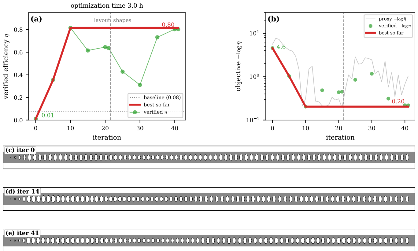
FIG. 2. Inverse-design trajectory. (a) Verified interface efficiency \eta from the periodic non-gradient (high-resolution time-domain) checks versus iteration: it climbs from 0.01 to 0.80, and the best-so-far envelope (red) shows that the optimizer reaches its final efficiency by the end of the layout stage, with the shape stage refining it. The dashed line marks the layout→shapes boundary; the dotted line is the hand-tuned baseline. (b) Optimization objective versus iteration: the verified interface loss -\log \eta from the non-gradient checks falls from 4.6 to 0.20, and its best-so-far envelope decreases monotonically to the delivered design. The faint trace is the proxy surrogate -\log \tilde{\eta} actually minimized at each iteration. The full proxy objective [Eq. (7)] additionally carries a resonance-penalty term whose transients are absorbed by the final trim and are not shown. (c)–(e) Top-view snapshots of the structure at early, intermediate, and final iterations, showing the evolving hole schedule.
