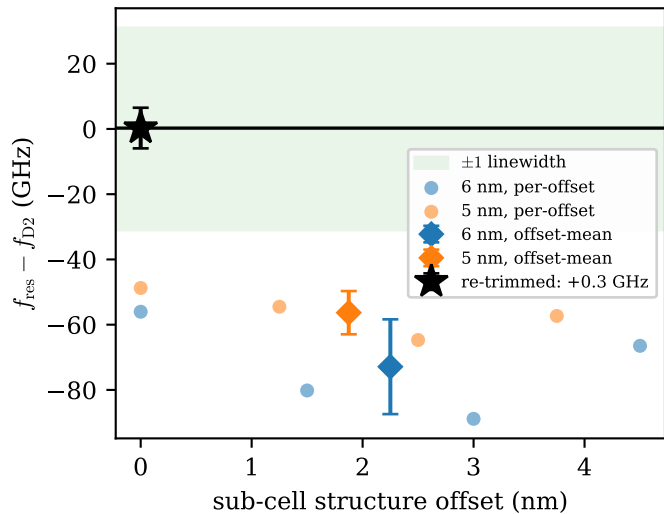
(b) grid-offset averaged + re-trim
