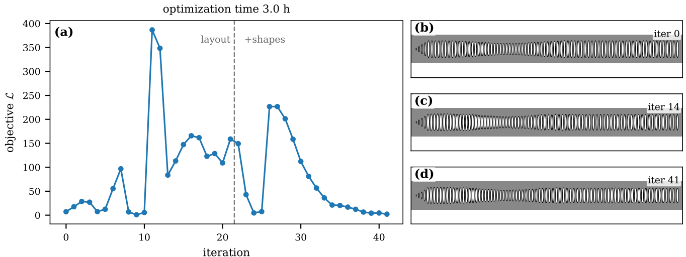
FIG. 3. Inverse-design trajectory. (a) Objective \mathcal{L} [Eq. (7)] versus iteration; the dashed line marks the layout \rightarrow shapes stage boundary. The mid-run excursion is the frequency penalty acting as the resonance temporarily drifts off target. (b)–(d) Top-view snapshots of the structure at early, intermediate, and final iterations, showing the evolving hole schedule.
