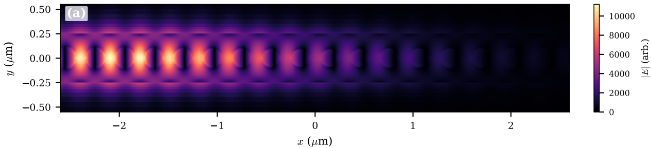
beam midplane ( z=0 )
