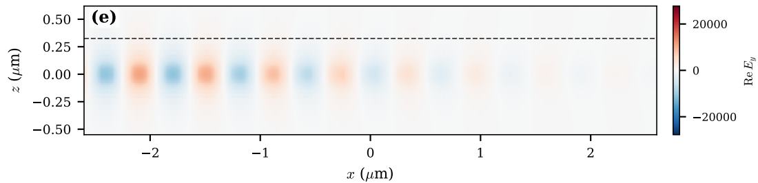
longitudinal ( y=0 ), \text{Re } E_y (standing wave)
