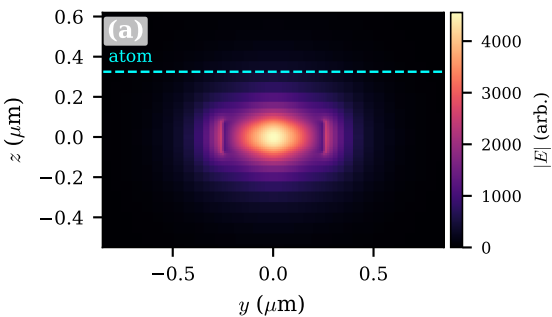
defect cut ( x=0 )
