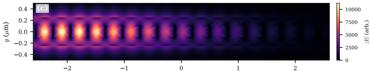
beam midplane ( z=0 )
