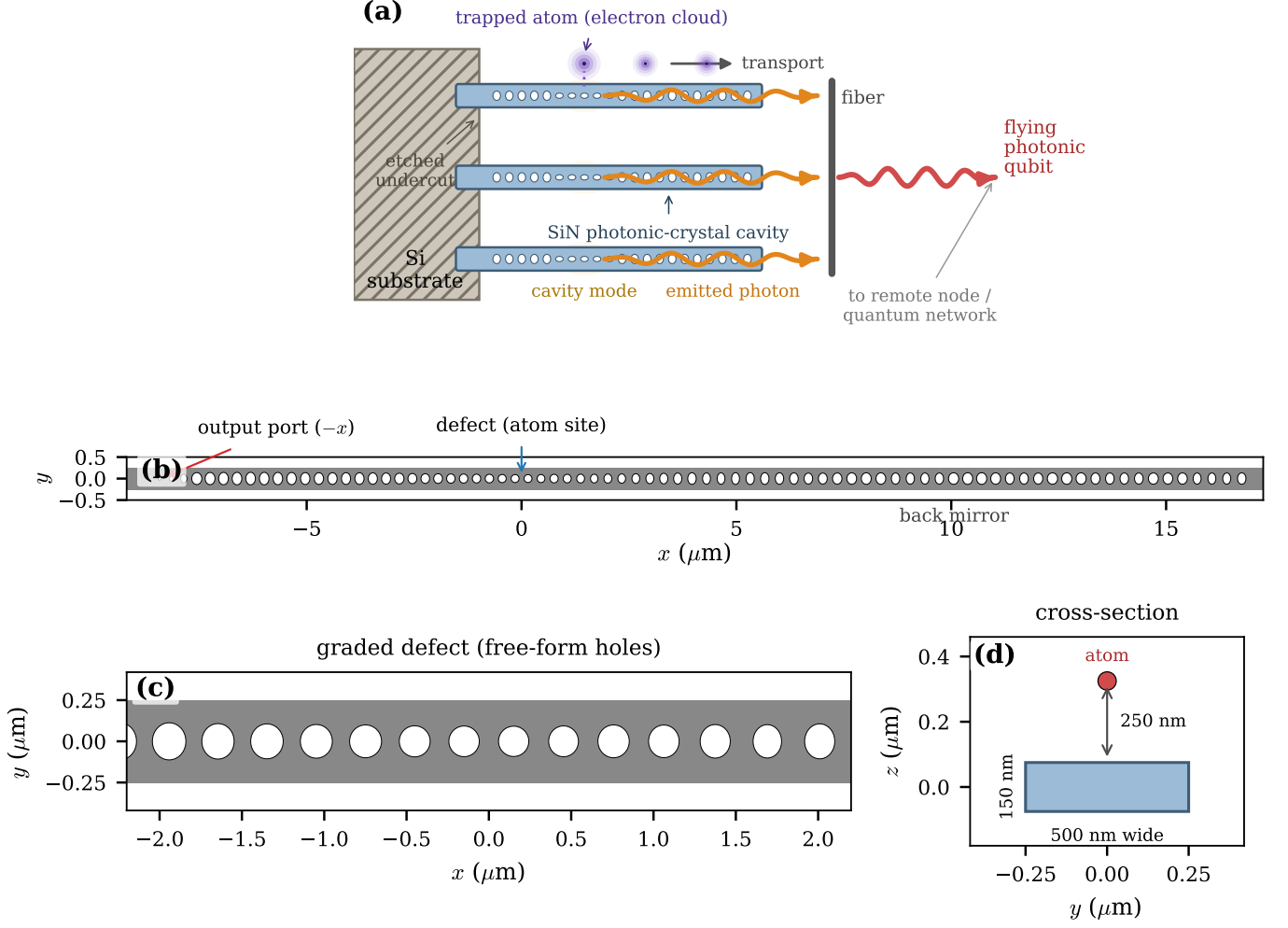
FIG. 2. Platform and final device. (a) Concept: an array of suspended SiN photonic-crystal “fingers” cantilevered beyond an etched substrate edge; tweezer-trapped atoms are transported over the series of cavities and transduced into flying photonic qubits collected into fiber. (b) Top view of the inverse-designed cavity, with the asymmetric output ( -x ) coupling mirror, the central defect (atom site), and the long back mirror. (c) Zoom of the graded defect region showing the free-form spline holes and the gentle lattice taper. (d) Beam cross-section: the 500 nm-wide, 150 nm-thick nanobeam with the atom trapped 250 nm above the top surface.
