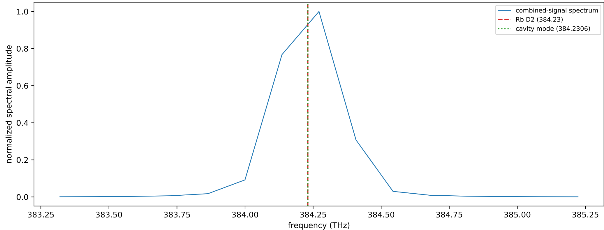
Mode isolation — single cavity mode; loaded linewidth \kappa/2\pi = 32.0 GHz
