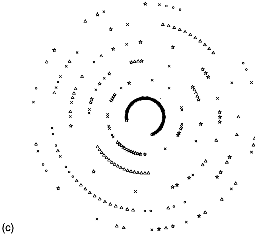
Fig. 4. Dependence of the escape time T on \alpha . Explanations are given in the text. Variations around m_1 , m_2 and m_3 are shown in (a), (b) and (c).
