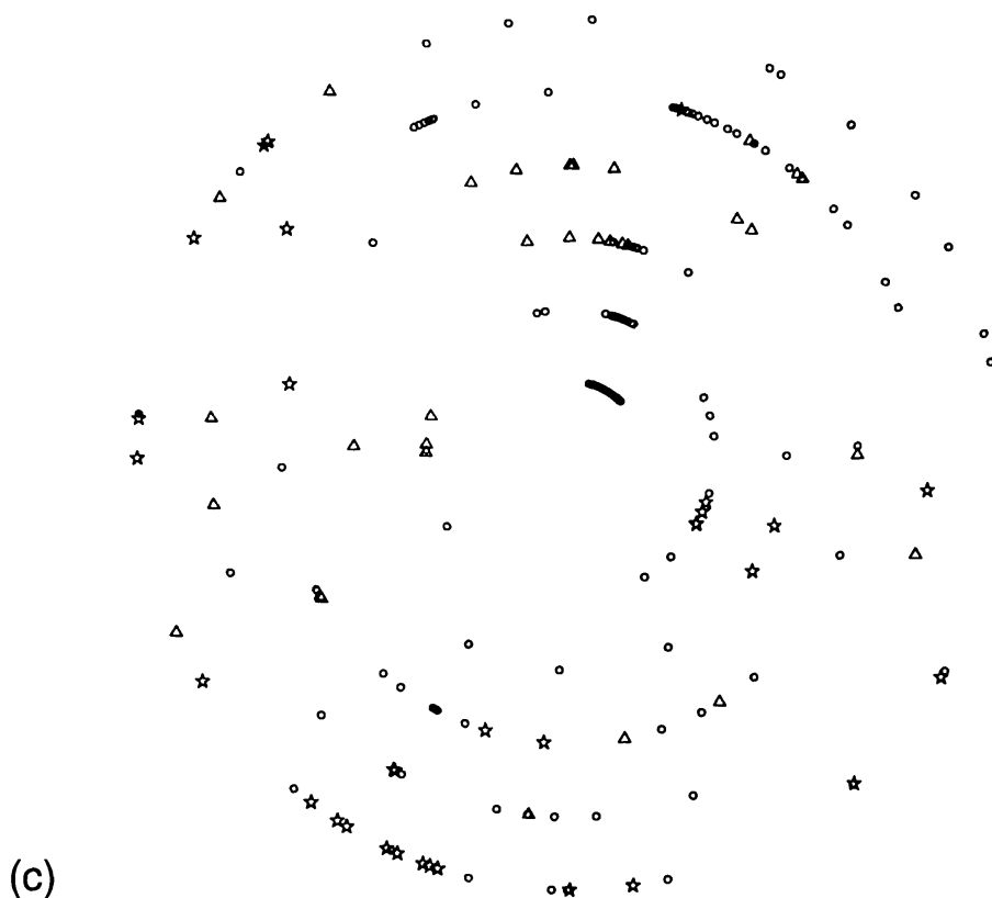
Fig. 2. Distributions of the angles of escape \beta for different values of initial deviations. The corresponding values of \delta_i from the innermost to the outermost circle are 5.0 \times 10^{-8} , 5.0 \times 10^{-7} , 5.0 \times 10^{-6} , 5.0 \times 10^{-5} , 5.0 \times 10^{-4} and 5.0 \times 10^{-3} . Results for deviations around m_1 , m_2 and m_3 are shown in (a), (b) and (c), respectively. Escape of components m_1 , m_2 or m_3 is denoted by circles, triangles and asterisks. The x-axis is horizontal.
