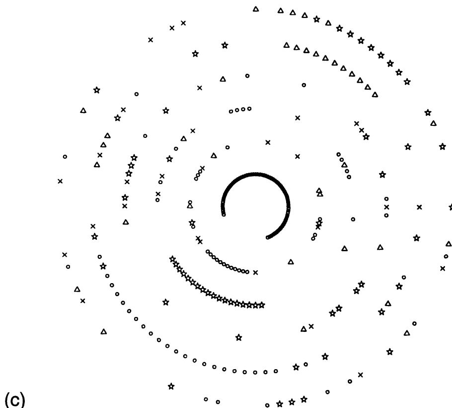
Fig. 3. Dependence of the escape angle \beta on the initial azimuth angle \alpha . Symbols are defined in the text. Variations around m_1 , m_2 and m_3 are shown in (a), (b) and (c).
