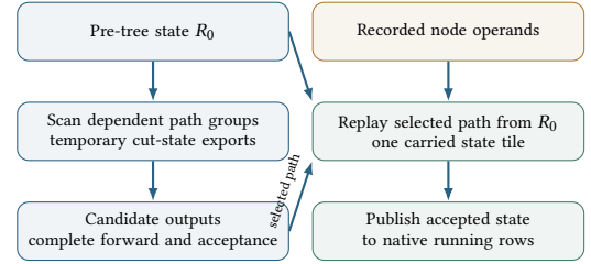
Figure 3: State lifetime in the path-scan verifier. Temporary cut states connect path groups; recorded operands support selected-path replay. Only the accepted frontier becomes native persistent state.
