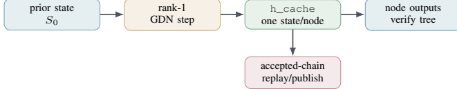
Fig. 4. The scan verifies all candidate nodes with parent-indexed recurrent state. Replay re-executes only the accepted chain and publishes durable GDN/conv state.
