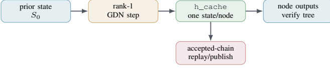
Fig. 3. The scan verifies all candidate nodes with parent-indexed recurrent state. Replay re-executes only the accepted chain and publishes durable GDN/conv state.
