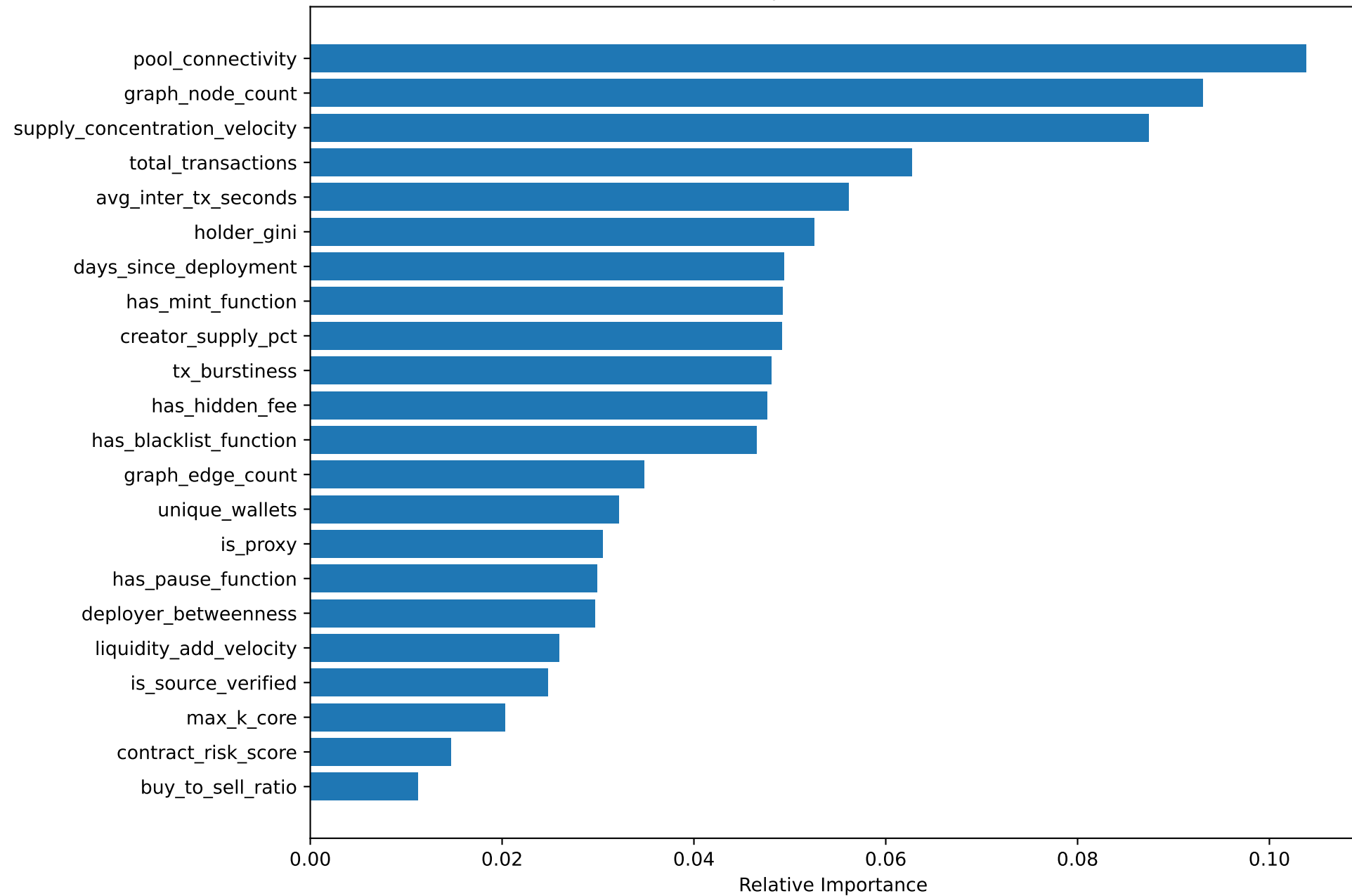
Global Feature Importance (XGBoost Baseline)
