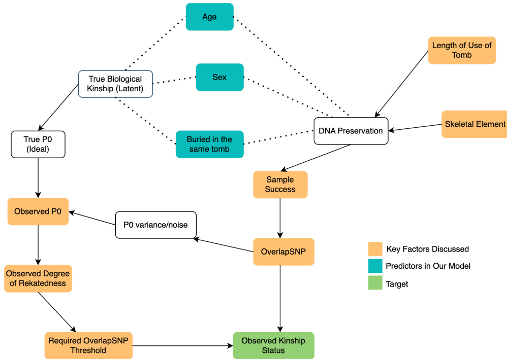
Figure 5: Directed Acyclic Graph (DAG)
