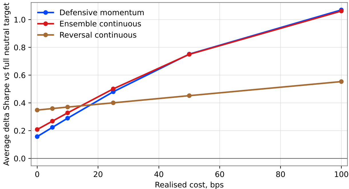
Transaction-cost sensitivity
