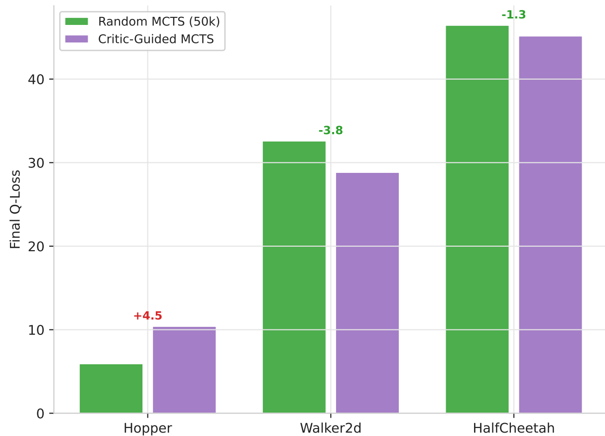
Phase 2 — Critic-Guided vs Random MCTS
