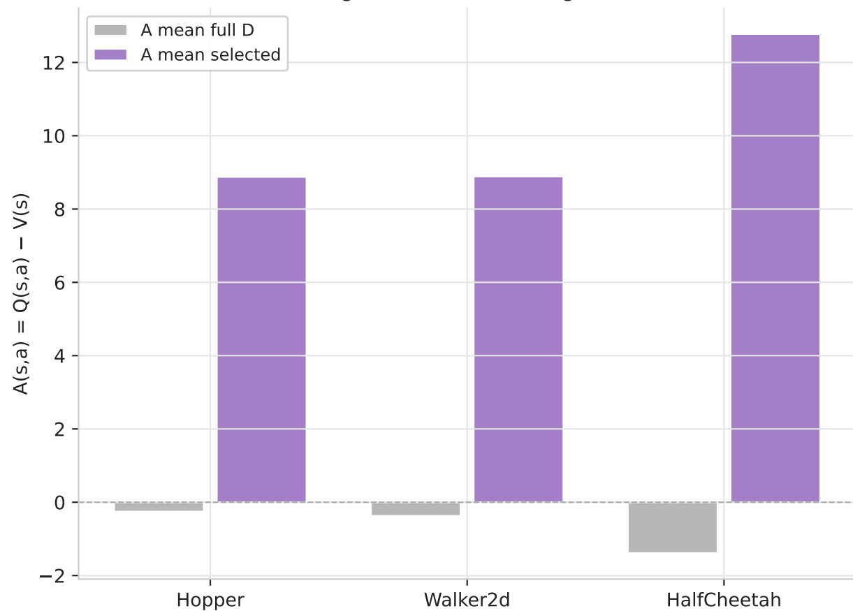
Critic-guided selection — high A(s,a)
