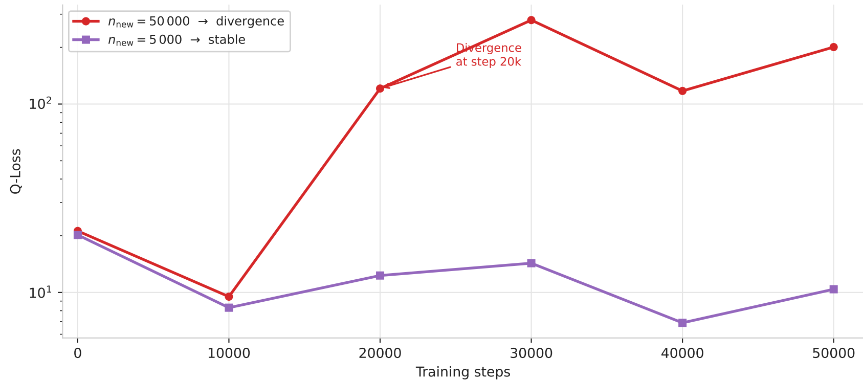
Q-Loss trajectory :Critic-Guided MCTS on Hopper Effect of augmentation volume ( n_{\text{new}} , warmup = 20\,000 steps)
