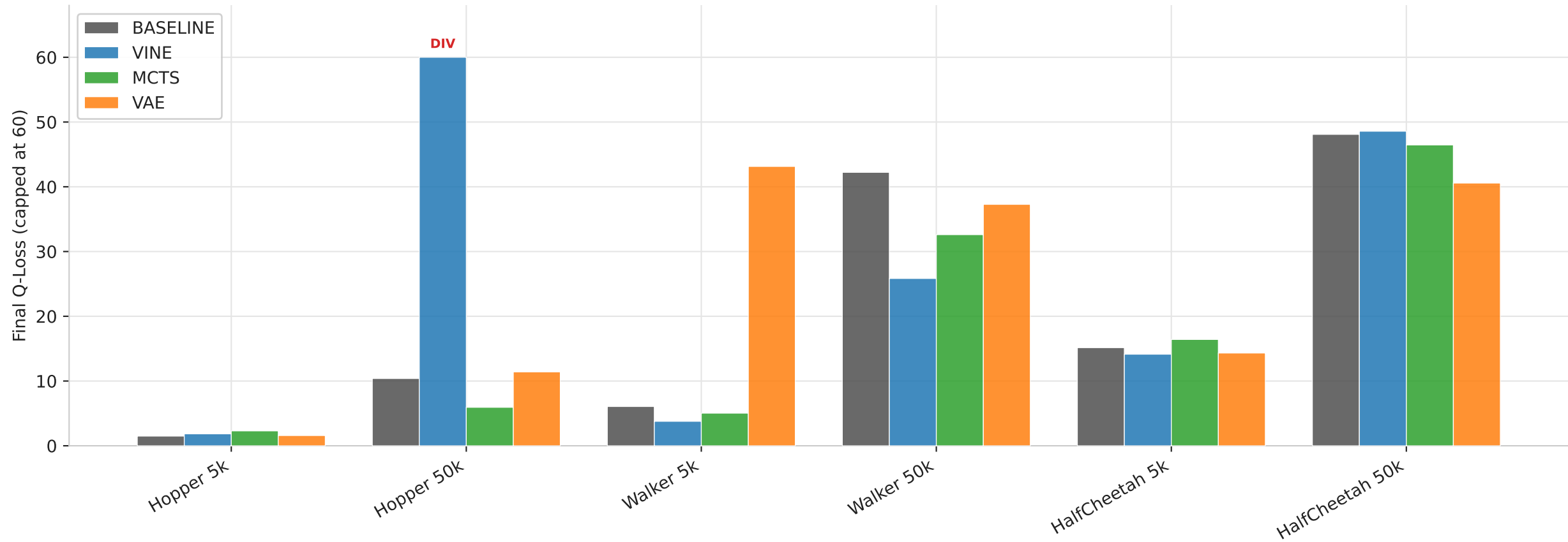
Phase 1 : Q-Loss Comparison: Vine / MCTS / VAE vs Baseline
