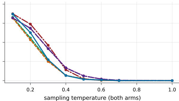
Sheared-LLaMA-2.7B
