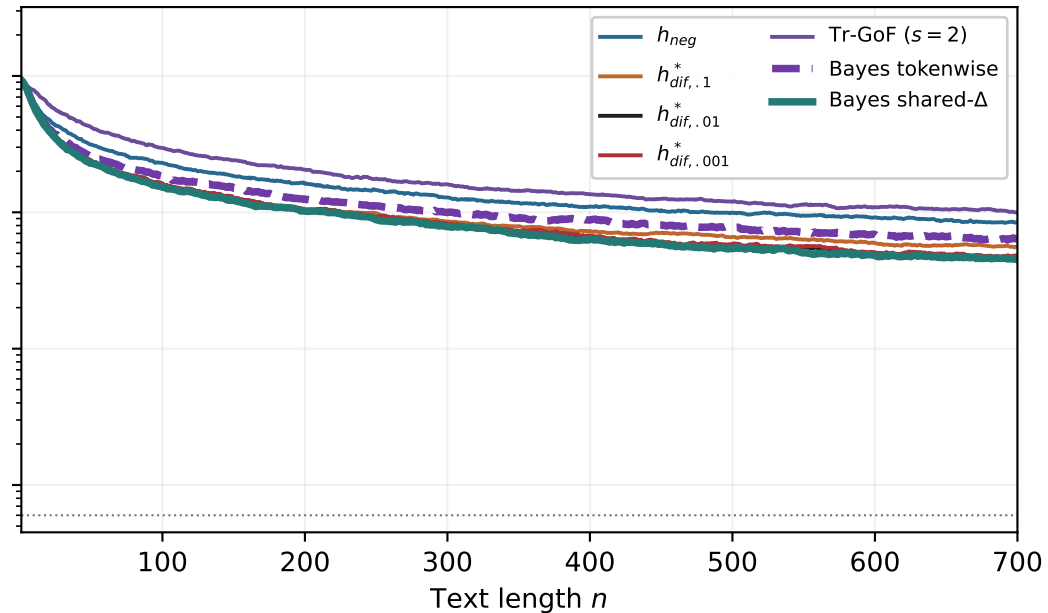
Inverse-transform watermark
