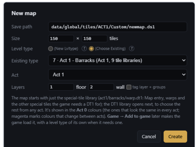
Map → New map, starting from an existing level type.
