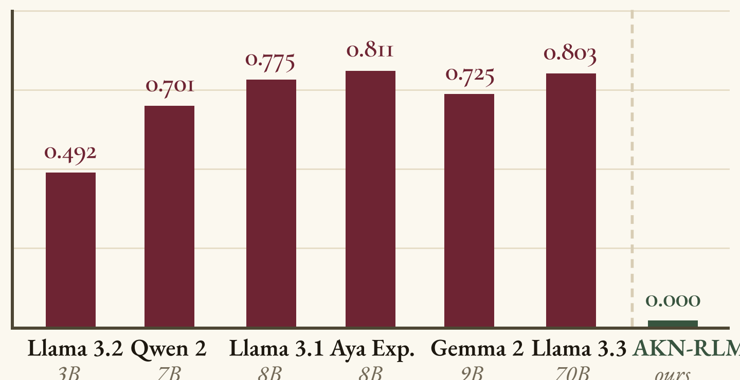
Fig. 1. Hallucinated-citation rate: the share of cited articles that do not exist , per direct-LLM baseline (244 questions). Scale does not help — the 70B model fabricates 4 of 5 citations. Gemini 2.5 reaches 0.008 only by declining to cite at all, and six of seven baselines import foreign law on >12 of 40 trap questions. AKN-RLM: 0.000.
