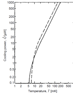
Figure 2.29: Cooling power as a function of temperature of a commercial ^3\text{He}-^4\text{He} dilution refrigerator, for two still heating powers: 8 mW (full line) and 22 mW (dashed line).
