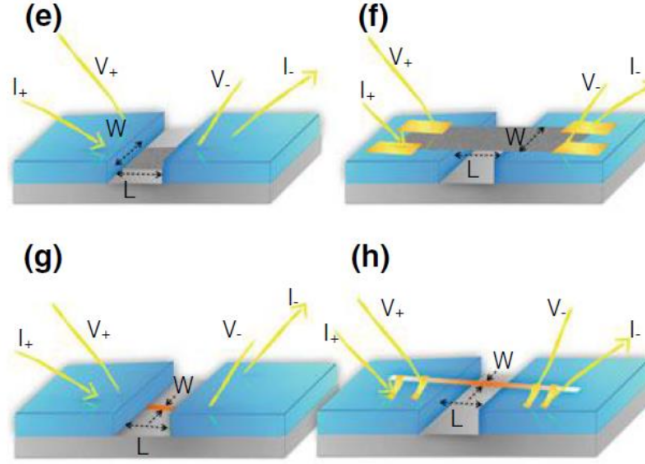
Figure 2.35: (e) A flake of graphene or a topological insulator used as a barrier. (f) A suspended nanowire deposited on the superconductor. (g) A nanowire as a barrier. (h) Suspended configuration with a trench separating the two electrodes. These configurations assemble pre-built blocks and may circumvent material science incompatibilities due to critical deposition conditions. The distance between the electrodes, L , is a critical parameter and must be of the order of the coherence length in N, \xi_n .
