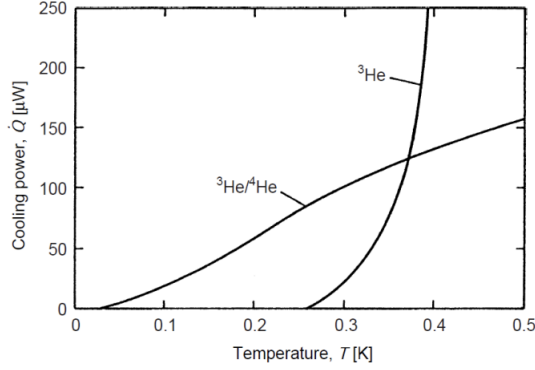
Figure 2.18: Cooling power of a ^3\text{He} evaporation cryostat and of a ^3\text{He} - ^4\text{He} dilution refrigerator, assuming that the same pump with a helium gas circulation rate of 5\text{ l s}^{-1} is used [7.9] (Diagram shows Cooling power, \dot{Q} [ \mu\text{W} ] vs. Temperature, T [K]. Curves labeled ^3\text{He}/^4\text{He} and ^3\text{He} )
