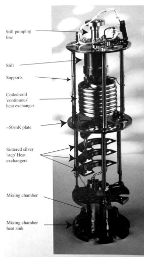
Figure 2.28: A modern dilution refrigerator. Courtesy of Oxford Instruments.
