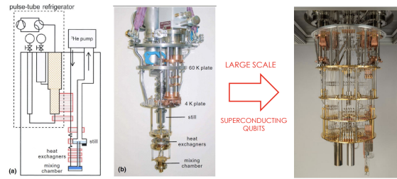
Figure 2.30: Schematic diagram (a) and photograph (b) of a dry dilution refrigerator precooled by a two-stage pulse tube cryocooler. On the right Example from S. Krinner et al. Engineering cryogenic setups for 100-qubit scale superconducting circuit systems EPJ Quantum Technol. 6, 2 (2019; Dilution Refrigerator Bluefors XLD400 with Pulse Tube Coolers (2x Cryomech PT 420))
