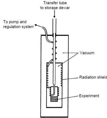
Figure 2.7: Evaporation cryostat for the temperature range T > 5K . A mixture of liquid and gaseous ^4\text{He} is transferred via a transfer tube from the storage dewar to the cryostat. The mixture is pumped through a spiral tube which is first connected to a chamber on which the experiment is mounted and then soldered to a radiation shield before it leaves the cryostat. The temperature of the experiment can be regulated by a heater and/or a valve which regulates the helium flow.
