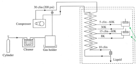
Figure 2.1: A simplified diagram of a Collins He liquefier showing flow rates typical of the original machine and early commercial models
