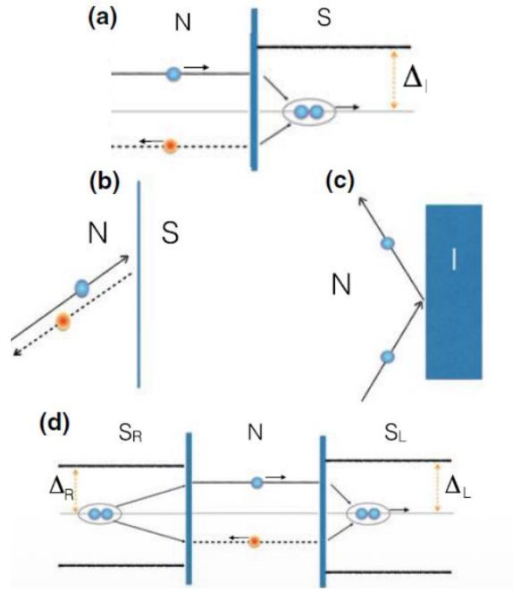
Figure 2.34: (a) Energy representation of the Andreev reflection (AR) process: an electron excitation slightly above the Fermi level in the normal metal is reflected at the interface as a hole excitation slightly below the Fermi level. (b) Spatial representation of AR at the S/N interface. (c) Spatial representation of normal reflection by an insulator. Normal reflection conserves charge but does not conserve momentum, while AR conserves momentum but does not conserve charge. The electron is reflected as a hole with the same momentum and opposite velocity. The missing charge of 2e is absorbed as a Cooper pair by the superconducting condensate. (d) Energy representation of Andreev reflections in SNS junctions.
