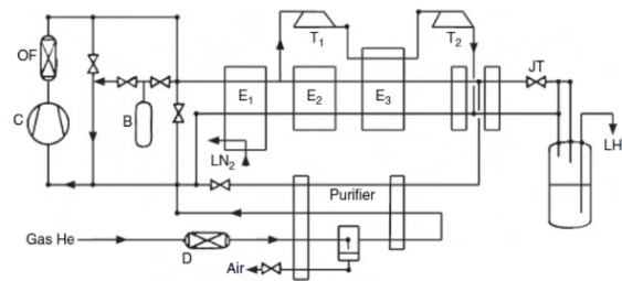
Figure 2.2: Flow diagram of the Linde TCF series of turbine helium liquefiers. C denotes the screw compressor, OF the oil filter, E_{1,2,3} the heat exchangers, T_{1,2} the turbo-expanders and JT the final Joule-Thomson stage. Cylinder B is for pure He gas storage and Gas He is the normal He gas input to the purifier.
