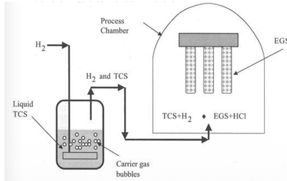
Figure 1.1: Siemens process
