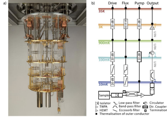
Figure 2.32: Cabled dilution refrigerator (DR). (a) Bluefors XLD DR with 25 drive lines, 25 flux lines, 4 read-out, 6 read-in, and 5 pump lines installed (see end of Sect. 3.1 for details). (b) Schematic of the cabling configuration within the DR
