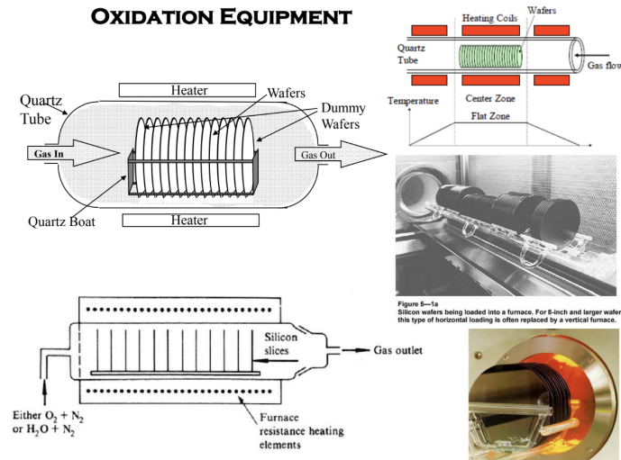
Figure 1.8: Oxidation Equipment
