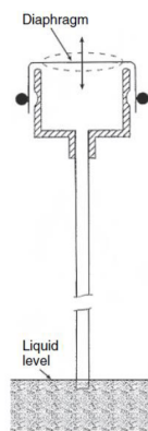
Figure 2.12: Level detector
