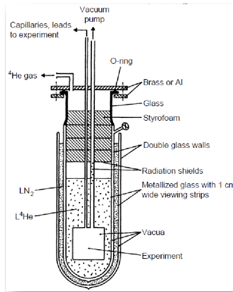
Figure 2.5: A double-walled glass dewar for LN_2 and L^4He . The inner surfaces of the glass are covered with aluminium or silver films to block thermal radiation (except for a vertical 1cm wide viewing strip). Four or five radiation baffles force the exiting cold gas to flow along the dewar walls, thus cooling it as well as the pumping tubes. The effectiveness of the baffles is increased by filling the spaces between them with Styrofoam.
