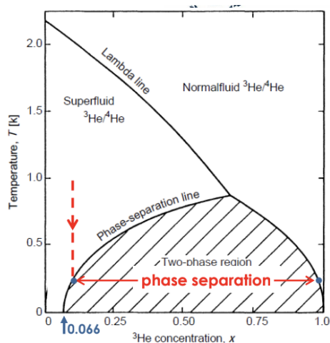
Figure 2.16: Phase diagram showing phase separation (Descriptive labels: 2.0 Temperature, T [K], 1.5, 1.0, 0.5, Lambda line, Normalfluid {}^3\text{He}/{}^4\text{He} , Superfluid {}^3\text{He}/{}^4\text{He} , Phase-separation line, Two-phase region, 0.066 {}^3\text{He} concentration, x )
