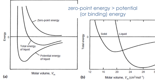
Figure 2.3: (a) Zero-point and potential energies of liquid ^4\text{He} as a function of molar volume. The total energy is the sum of these two energies. (b) The illustration of why the liquid state is the stable one for helium at saturated vapour pressure even at the T = 0\text{K} .
