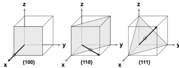
Figure 1.4: Common cubic crystal planes illustrated are \{100\} , \{110\} , and \{111\} .
