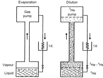
Figure 2.20: Gedanken experiment for comparison of a helium evaporation refrigerator and a ^3\text{He} – ^4\text{He} dilution refrigerator (Diagram shows components: Vapour, Liquid, Evaporation ( \uparrow ), Gas pump ( \downarrow ), Dilution ( \uparrow ), ^3\text{He} pump, 1K, ^3\text{He} – ^4\text{He} , ^3\text{He} )
