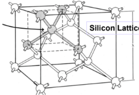
Figure 1.3: Silicon lattice. Gray spheres denote the corners of a tetrahedron
