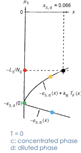
Figure 2.17: Diagram illustrating chemical potential ( \mu ) vs. concentration ( x ). (Labels: \mu_3 , x_{3,d} = 0.066 , 0 , x , -L_3/N_0 , -\epsilon_{3,d}(x) + k_B T_F(x) , -\epsilon_{3,d}(0) , -\epsilon_{3,d}(x) , T = 0 , c: concentrated phase, d: diluted phase, ^3\text{He} in Pure ^3\text{He} ( x = 1 ))
