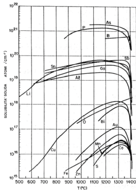
Figure 1.5: A graph detailing Solid Solubility (ATOMI/cm 3 ) versus Temperature ( T(^{\circ}C) ) shows solubility profiles for various elements (As, P, B, Sb, Sn, Ga, Al, Li, Bi, Au, Mn, Co, Cu, S, Fe, Zn).
