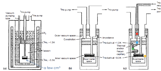
Figure 2.13: Cryostat with external pump: ^3\text{He} cryostats of increasing sophistication. (a) Non-recirculating ^3\text{He} refrigerator with a pumped main ^4\text{He} bath. (b) Non-recirculating ^3\text{He} refrigerator with a continuously operating ^4\text{He} evaporator. (c) Recirculating ^3\text{He} refrigerator with a continuously operating ^4\text{He} evaporator
