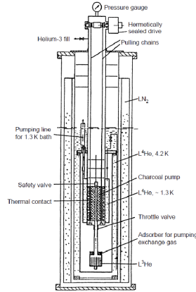
Figure 2.14: cryostat with a hermetically sealed ^3\text{He} system, reaching 0.25K. The charcoal pump can be raised or lowered by means of a chain drive operated via a hermetically closed rotating seal
