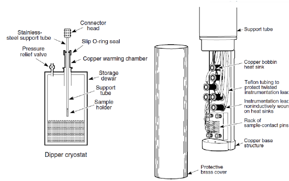
Figure 2.8: Sample-holder section of a dipper probe, showing copper base structure and sample holder for temperature stability, and copper-bobbin heat-sinking arrangement for the instrumentation leads
