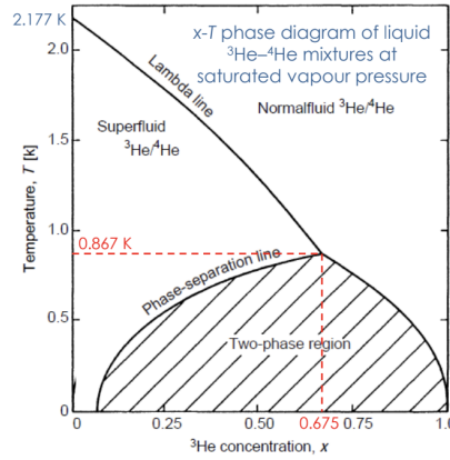
Figure 2.15: x - T phase diagram of liquid {}^3\text{He} - {}^4\text{He} mixtures at saturated vapour pressure (Descriptive labels: Si 2.177 kelvin, 2.0 Temperature, 1.5, Lambda line, Normalfluid {}^3\text{He}/{}^4\text{He} , 1.0, Superfluid {}^3\text{He}/{}^4\text{He} , 0.5, Si 0.867 kelvin, Phase-separation line, Two-phase region, 0.25, 0.50, 0.675, 0.75, 1.00 {}^3\text{He} concentration, x )
