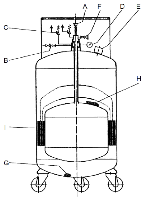
Figure 2.10: Commercial storage vessel for liquid {}^4\text{He} (A: connection for transfer tube, B: overflow valve, C: safety valve, D: manometer, E: vacuum and safety valves, F: gas valve, G: getter material, H:adsorbent material to maintain and improve the vacuum, I: superinsulation only partly shown).
