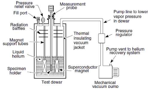
Figure 2.4: Schematic of an immersion measurement probe in a cryogenic liquid with a vacuum pump for lowering the boiling temperature of the cryogen bath.
