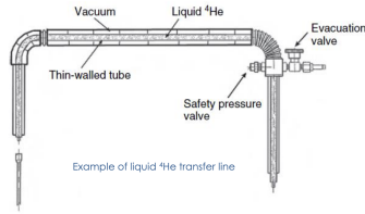
Figure 2.11: Transfer tube
