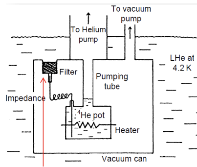
Figure 2.9: Cryostat with Variable Temperature for 1.3\text{K} \leq T \leq 4.2\text{K}
