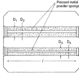
Figure 2.25: Diagram of a sintered metal powder step exchanger.
