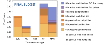
Figure 2.33: Total heat load budget for the operation of a 50 qubit processor. Predicted passive and active heat loads for the operation of a 50 qubit processor with individual drive and flux control. The heat loads are normalized to the measured cooling powers as presented in Table 2.5
