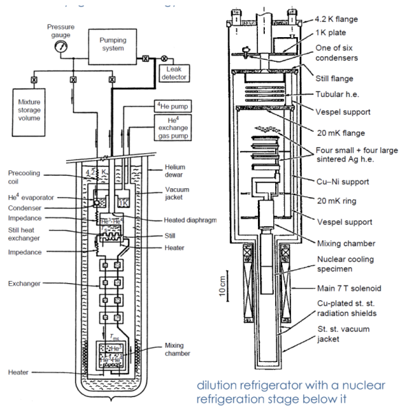
Figure 2.27: Schematic diagrams of successful “home-made” dilution refrigerators
