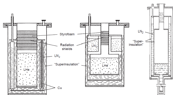
Figure 2.6: Metal Dewar
