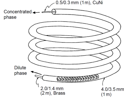
Figure 2.24: Diagram of a continuous counterflow heat exchanger.
