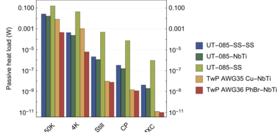
Figure 2.31: Heat flow for indicated cable types. Heat flow to the five temperature stages for indicated cable types and given cable lengths.
