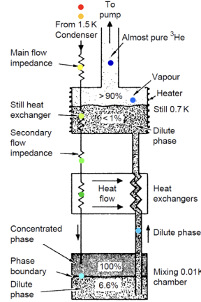
Figure 2.21: Schematic diagram of the dilution refrigerator circuit showing: To pump, From 1.5 K Condenser, Almost pure ^3\text{He} , Main flow impedance, Still heat, Vapour, Heater, Still 0.7 K, > 90\% , < 1\% , Secondary flow impedance, Heat exchangers, Dilute phase, Concentrated phase, Phase boundary, 100\% , 6.6\% , Mixing chamber 0.01K, Dilute phase
