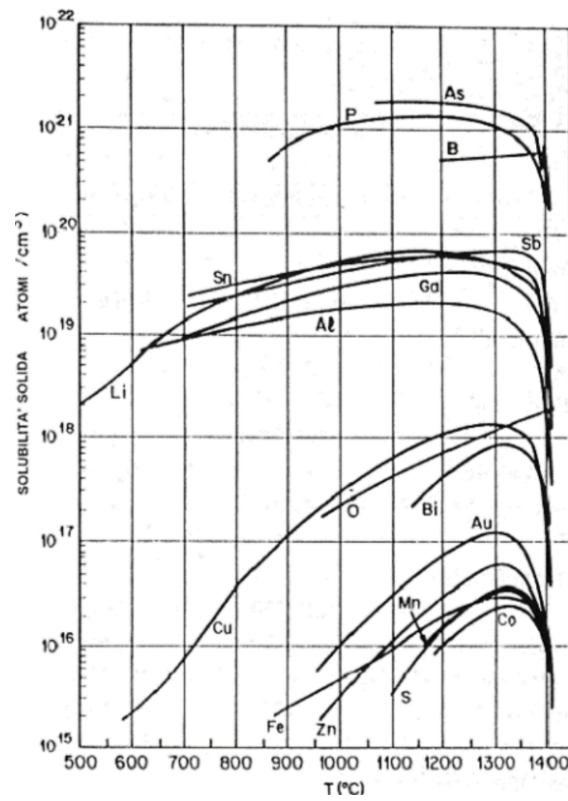
Figure 2.4: A graph detailing Solid Solubility (ATOMI/cm 3 ) versus Temperature ( T(^{\circ}C) ) shows solubility profiles for various elements (As, P, B, Sb, Sn, Ga, Al, Li, Bi, Au, Mn, Co, Cu, S, Fe, Zn).
