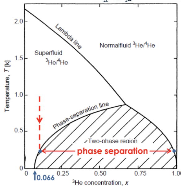
Figure 18.2: Phase diagram showing phase separation (Descriptive labels: 2.0 Temperature, T [K], 1.5, 1.0, 0.5, Lambda line, Normalfluid ^3\text{He}/^4\text{He} , Superfluid ^3\text{He}/^4\text{He} , Phase-separation line, Two-phase region, 0.066 ^3\text{He} concentration, x )
