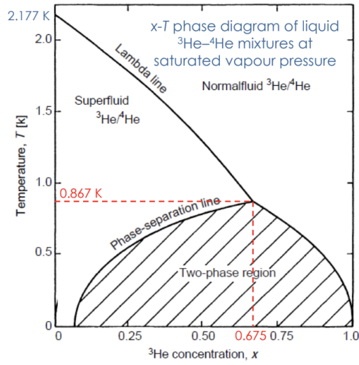
Figure 18.1: x - T phase diagram of liquid ^3\text{He} - ^4\text{He} mixtures at saturated vapour pressure (Descriptive labels: Si 2.177 kelvin, 2.0 Temperature, 1.5, Lambda line, Normalfluid ^3\text{He}/^4\text{He} , 1.0, Superfluid ^3\text{He}/^4\text{He} , 0.5, Si 0.867 kelvin, Phase-separation line, Two-phase region, 0.25, 0.50, 0.675, 0.75, 1.00 ^3\text{He} concentration, x )
