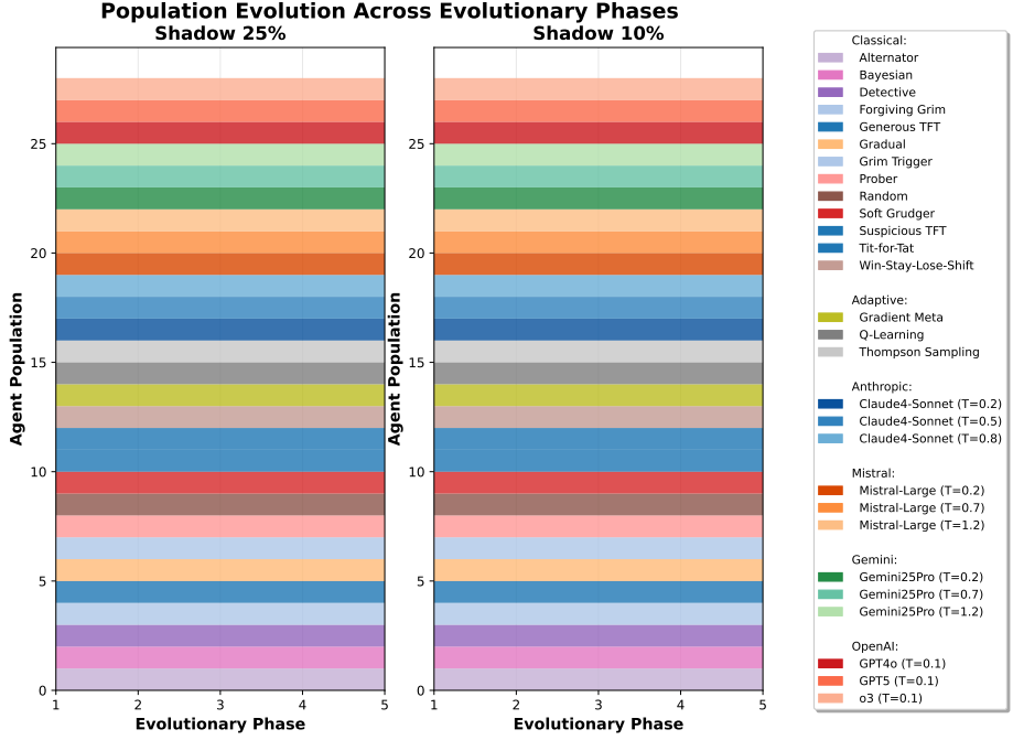
Fig. 2: Population Evolution 25% and 10% shadow length
