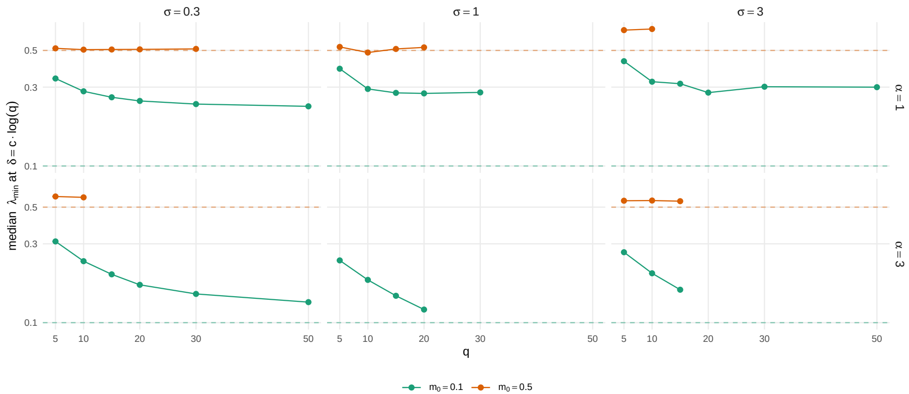
B. Verification: median at the extracted \delta = c \log q
