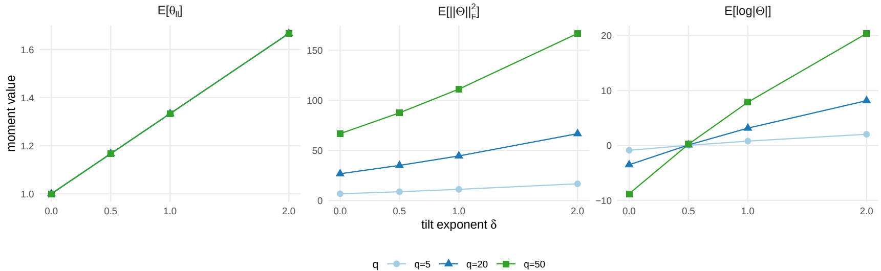
Empty-graph moments: closed-form (lines) vs empirical (points)
