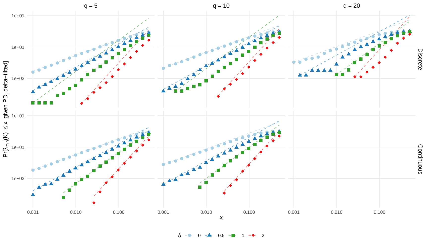
Empirical tail bound vs the x^{(\delta+1)} upper envelope (dashed)
