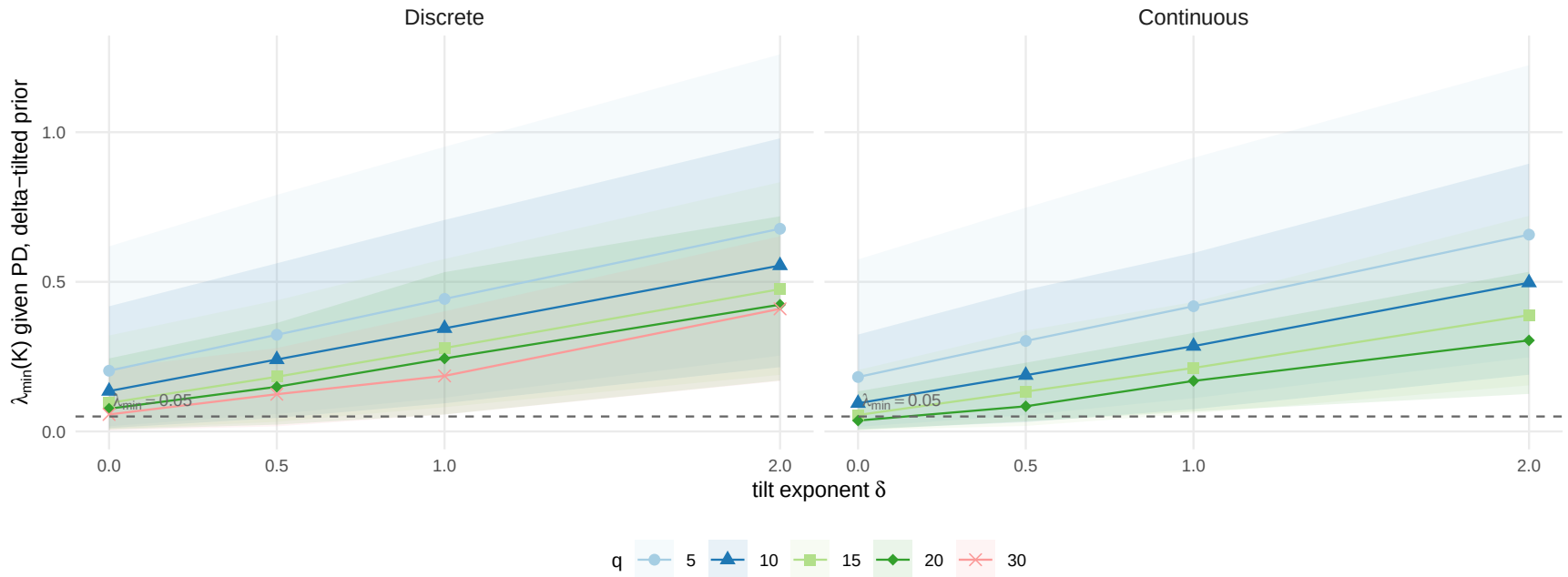
Tilt-only effect on the bulk of the PD-conditional prior (rejection-sampled)
