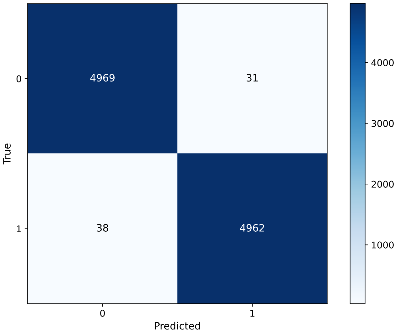
codebert confusion matrix
