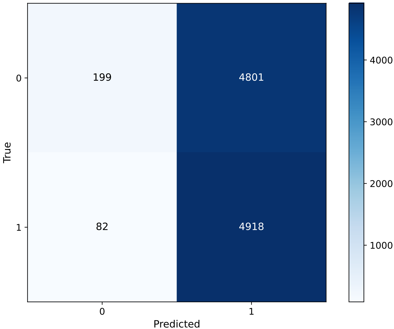
tfidf confusion matrix
