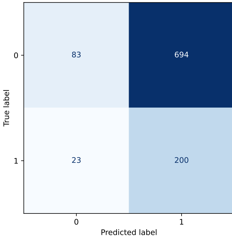
Confusion Matrix — Model C (Proposed) on Test Set
