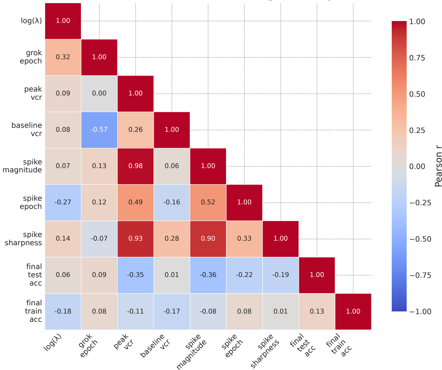
Metric Correlation Matrix (Grokking Runs Only)
