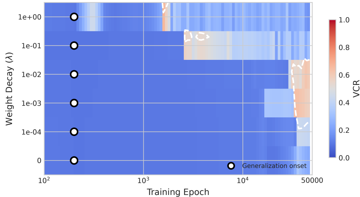
Phase Diagram: Transformer + ADAMW + Discrete
