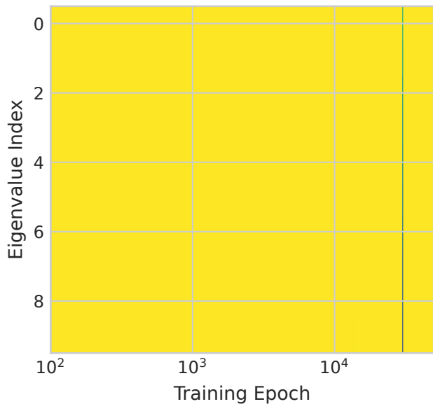
Transformer
