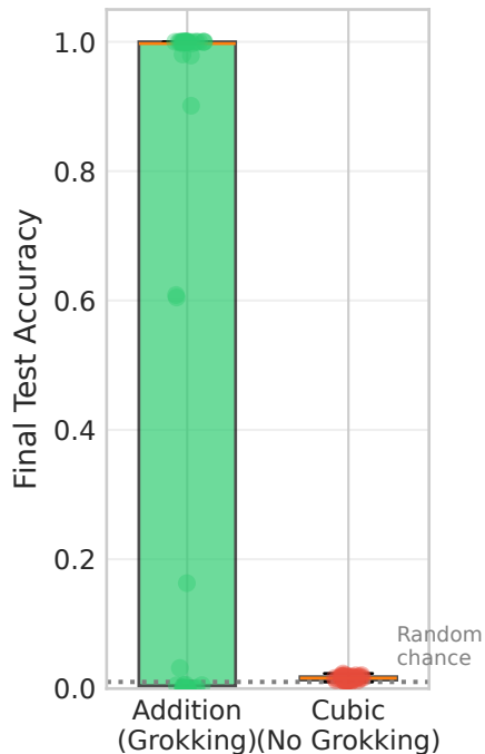
B. Test Accuracy by Task
