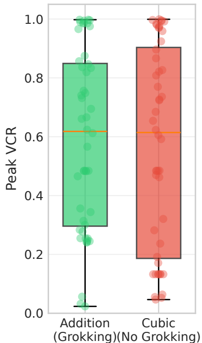
A. Peak VCR by Task
