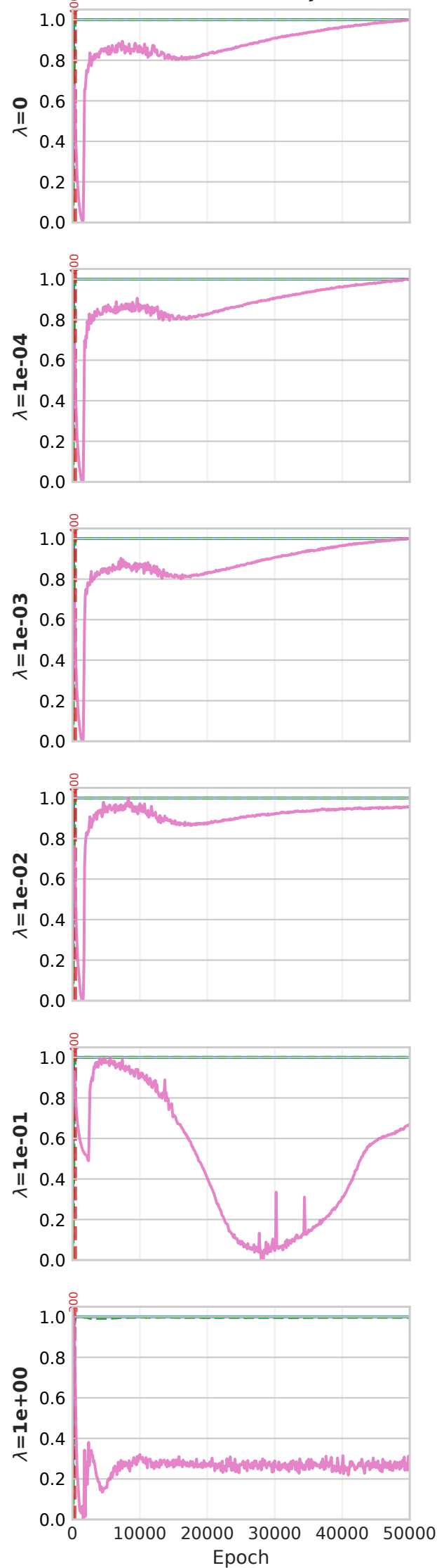
Addition: x + y
