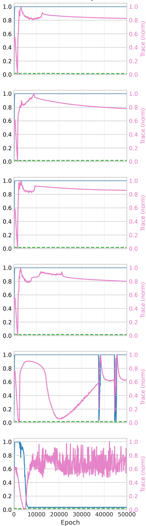
Cubic: x^3 + xy
