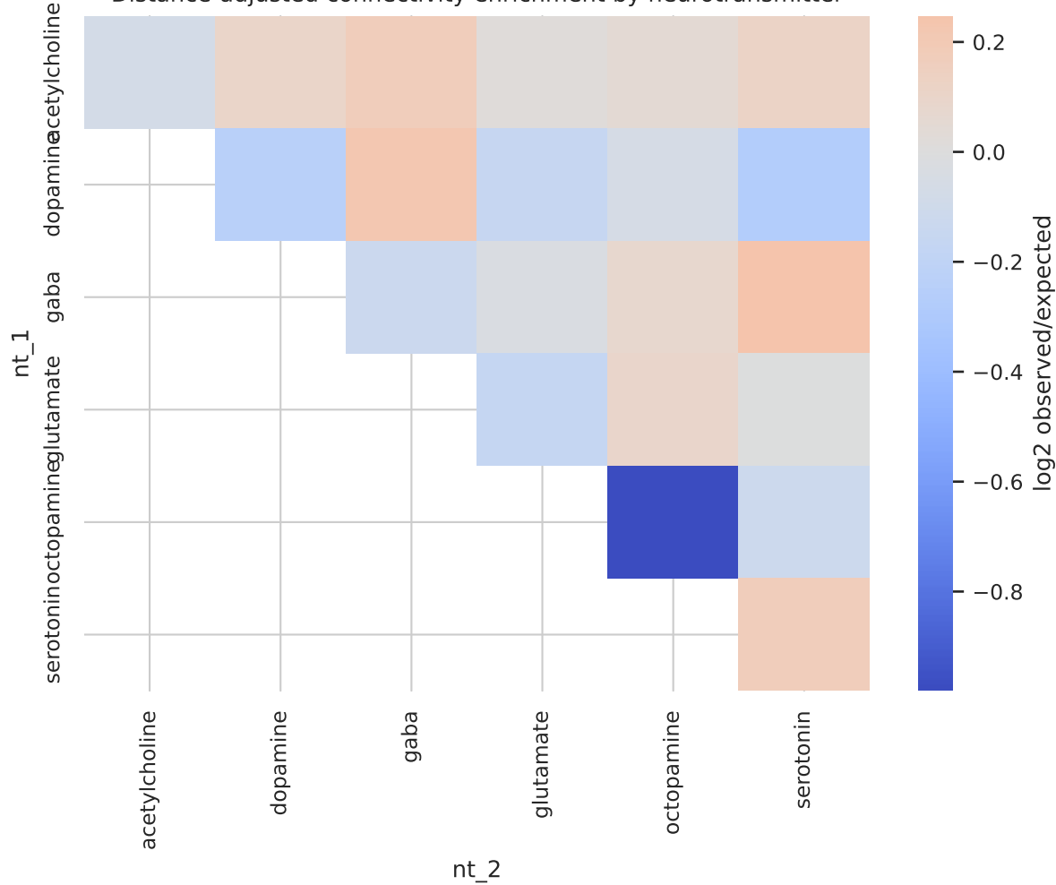
Distance-adjusted connectivity enrichment by neurotransmitter
