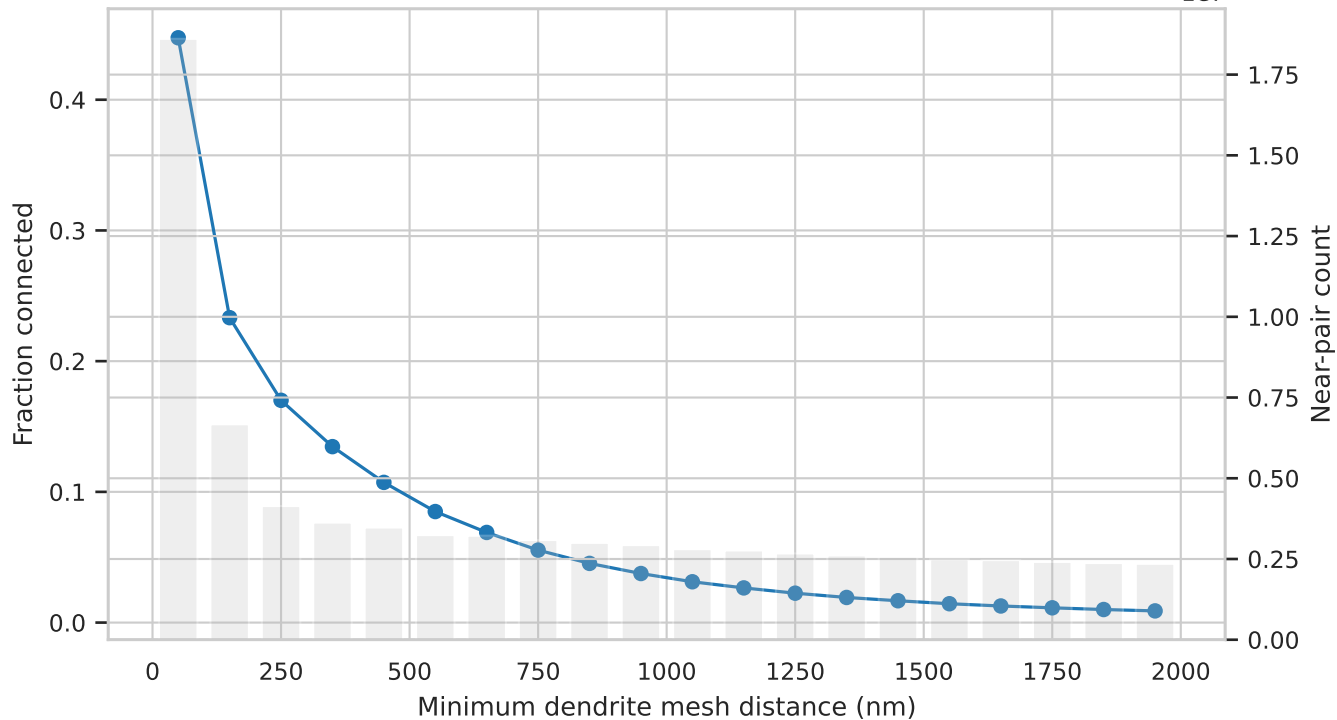
Connectivity falls sharply with dendrite-mesh distance
