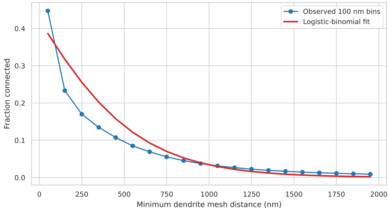
Fitted quantitative rule for distance-dependent connectivity
